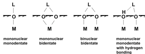
Figure 1. Illustration of mononuclear and binuclear (inner-sphere) complexes of adsorbed metal ions on a surface. See binuclear complex. From Maurice (2009), with permission.
